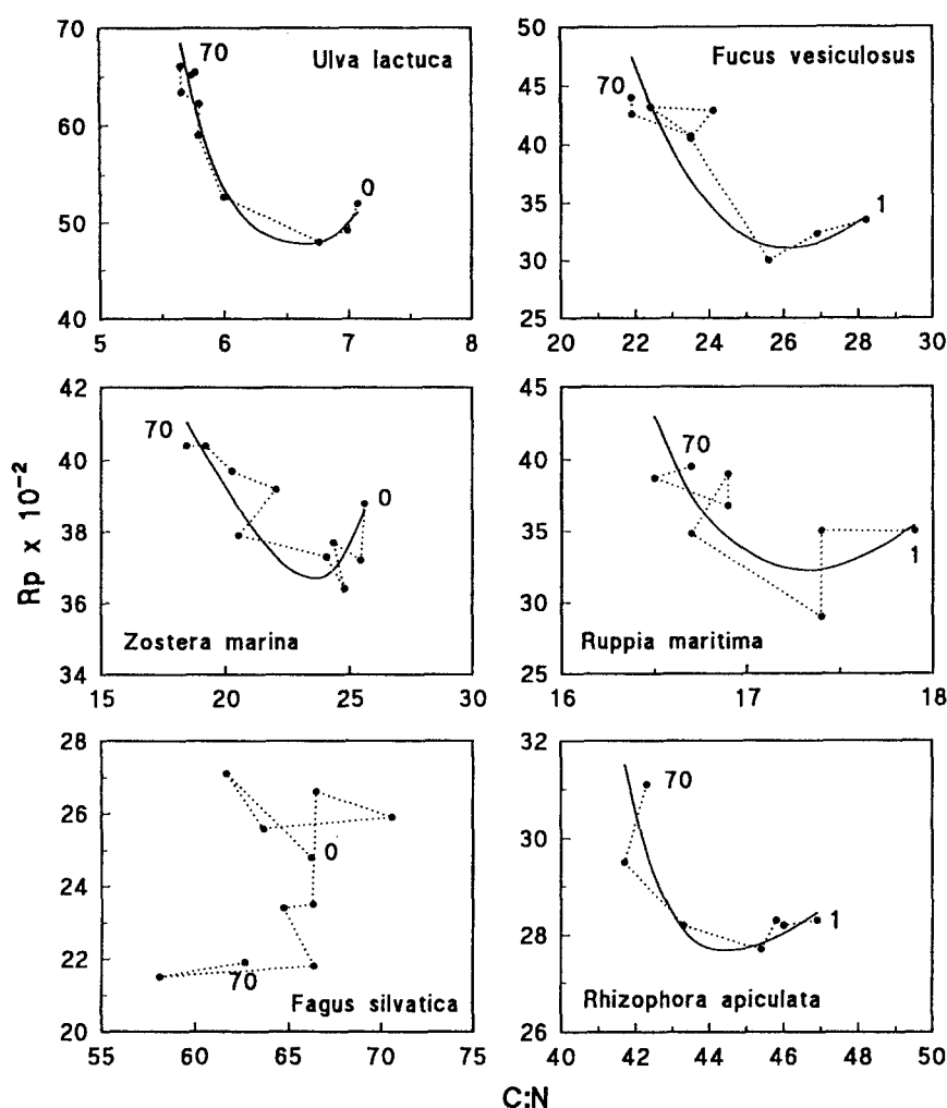
Fig. 6. Temporal relationships between the R_p index and C:N ratio of 6 different plant materials being decomposed aerobically in batch cultures. Dotted lines indicate the sequence of time points from the first (0 or 1) to the last sampling day (70). Smooth curves are drawn by eye.
