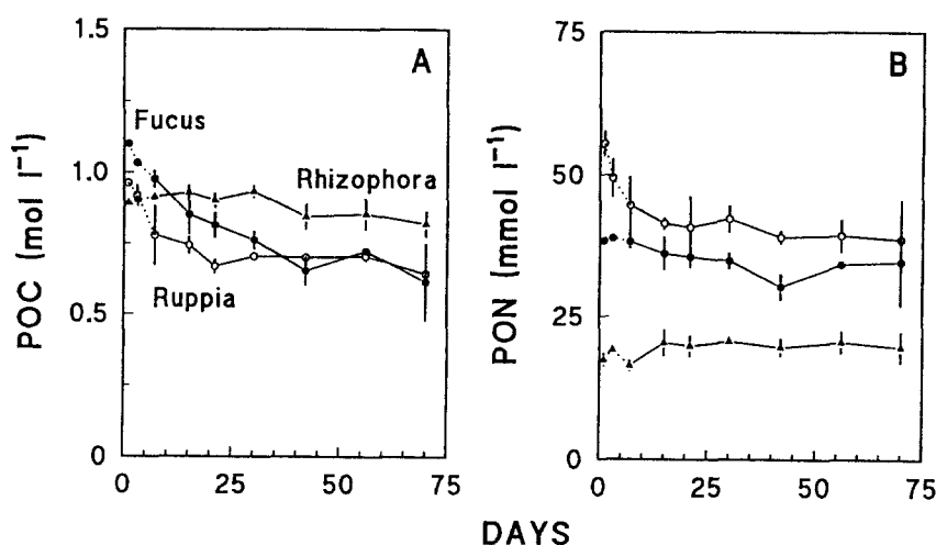
Fig. 2. Fucus vesiculosus , Ruppia maritima and Rhizophora apiculata . Temporal changes of (A) POC and (B) PON content in batch cultures over 70 days. Error bars indicate range of 2 cultures. Dotted lines represent the leaching phase (not included in estimates of first order decay constants).
