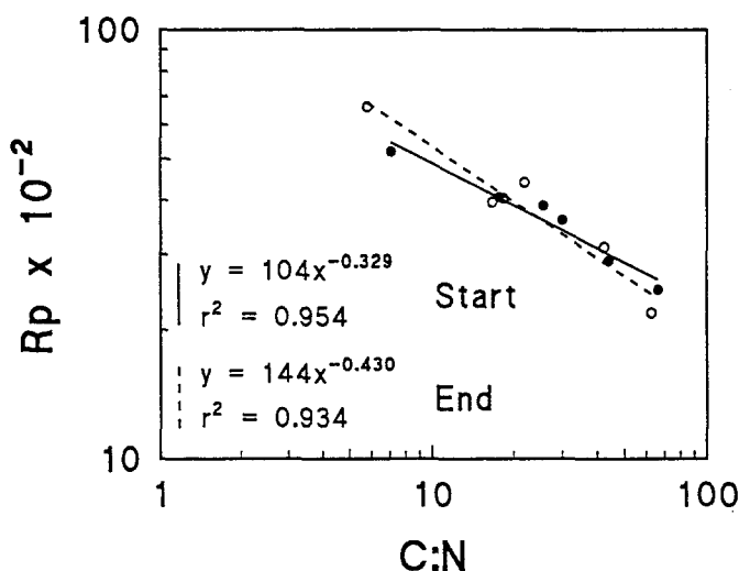
Fig. 7. The relationship between R_p index and C:N for the 6 plant materials examined, before (Start) and after (End) the 70 day decomposition period in batch cultures. Equations obtained by least squares linear regression are given.
