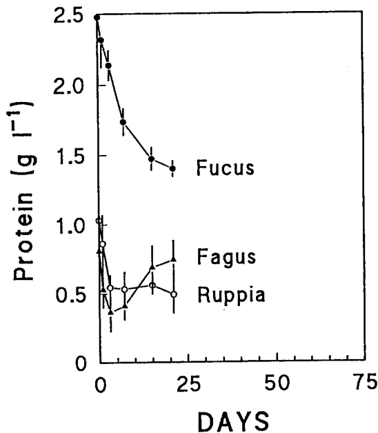
Fig. 3. Fucus vesiculosus , Ruppia maritima and Fagus silvatica . Temporal changes of protein content in batch cultures over 21 days. Error bars indicate \pm S.D. of 5 determinations on pooled samples from 2 cultures.
