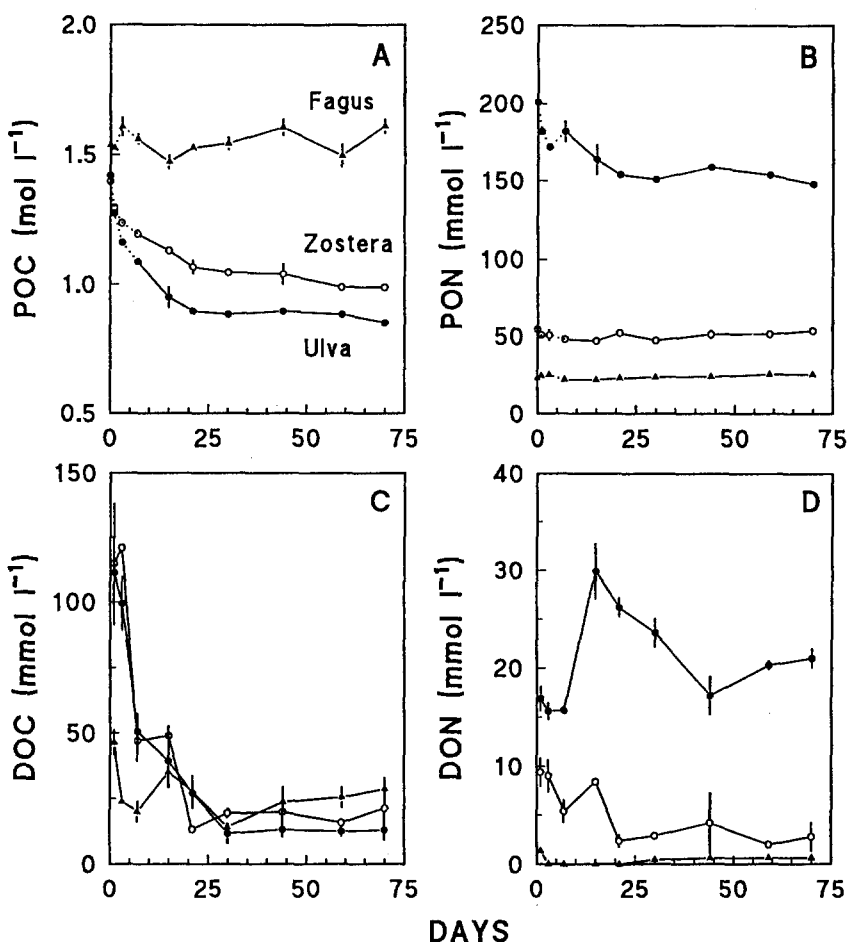
Fig. 1. Ulva lactuca , Zostera marina and Fagus silvatica . Temporal changes of (A) POC, (B) PON, (C) DOC and (D) DON content in batch cultures over 70 days. Error bars indicate range of 2 cultures. Dotted lines in (A) and (B) represent the leaching phase (not included in estimates of first order decay constants).
