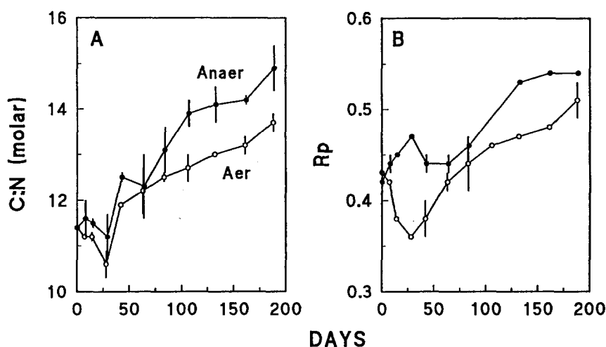
Fig. 9. Aerobic (Aer) and anaerobic (Anaer) sediment. Temporal changes of (A) C:N ratio (molar) and (B) Rp index in batch cultures over 190 days. Error bars indicate \pm S.D. of 4 cultures.
