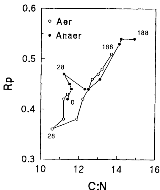
Fig. 10. Temporal relationships between the Rp index and C:N ratio of sediment detritus being decomposed under aerobic (Aer) and anaerobic (Anaer) conditions in batch cultures. Numbers shown represent the first (0), an intermediate (28) and the last sampling day (188).
