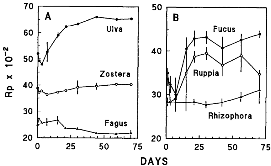
Fig. 5. Temporal changes of Rp index in batch cultures over 70 days. (A) Ulva lactuca , Zostera marina and Fagus sylvatica ; (B) Fucus vesiculosus , Ruppia maritima and Rhizophora apiculata . Error bars indicate range of 2 cultures.
