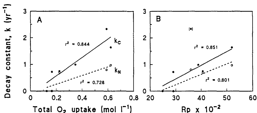
Fig. 11. The relationship between decay constants (carbon ( k_C ) and nitrogen ( k_N )) and (A) total time integrated oxygen uptake and (B) the initial Rp index of various plant materials being decomposed for 70 days. Lines are obtained by least squares linear regression. Correlation coefficients are given. Fucus vesiculosus is excluded from the carbon regression analysis in (B) because of an anomalous low Rp relative to k_C .
