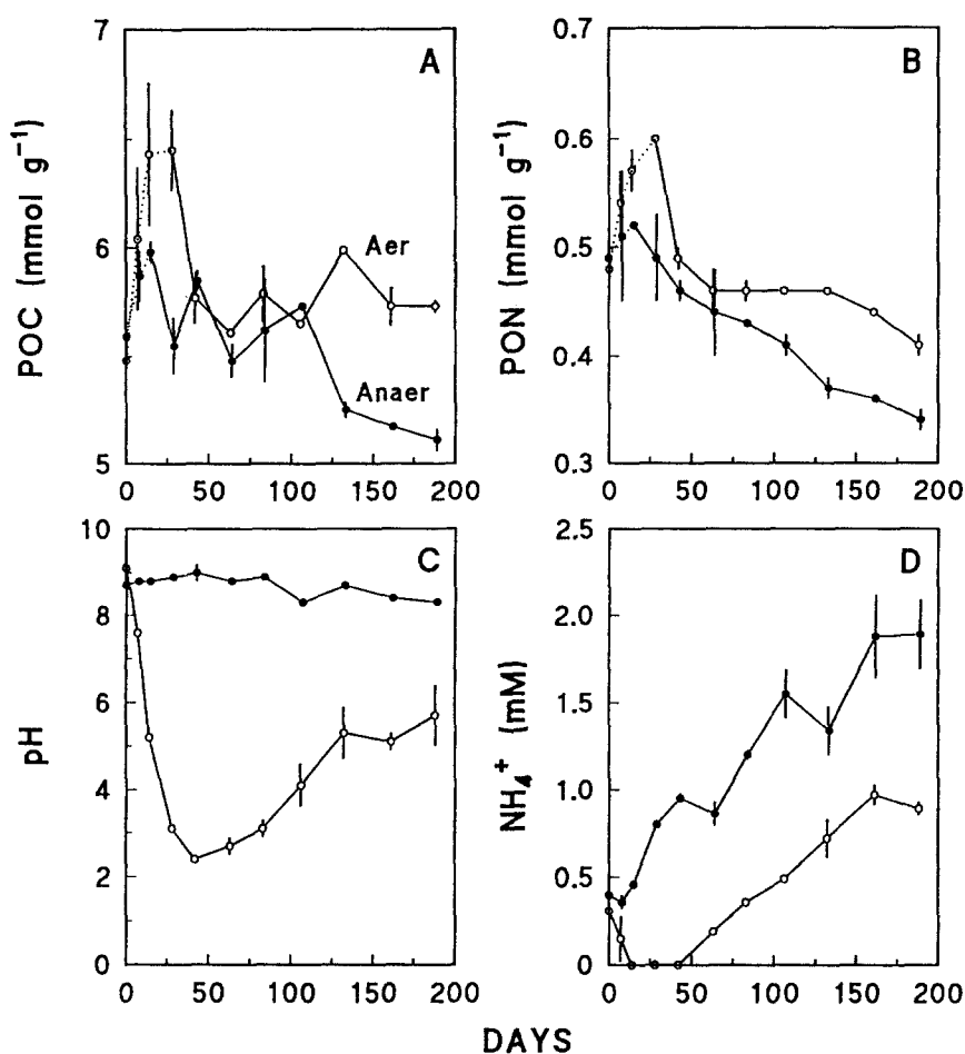
Fig. 8. Aerobic (Aer) and anaerobic (Anaer) sediment. Temporal changes of (A) POC, (B) PON, (C) pH and (D) \text{NH}_4^+ in batch cultures over 190 days. Error bars indicate \pm S.D. of 4 cultures. Dotted lines in (A) and (B) represent the organic enrichment phase (not included in estimates of first order decay constants).
