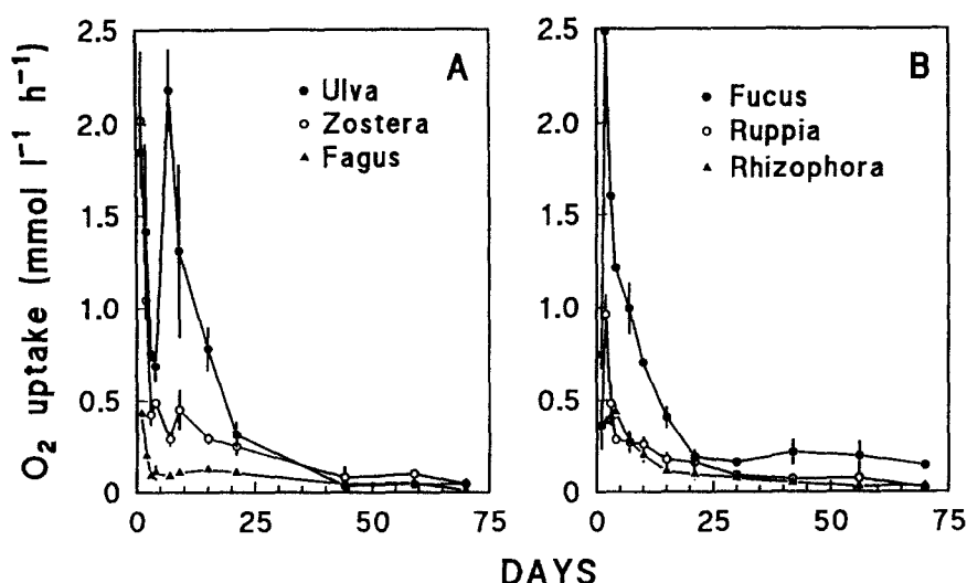
Fig. 4. Temporal changes of oxygen uptake in batch cultures over 70 days. (A) Ulva lactuca , Zostera marina and Fagus silvatica ; (B) Fucus vesiculosus , Ruppia maritima and Rhizophora apiculata . Error bars indicate range of 2 cultures.
