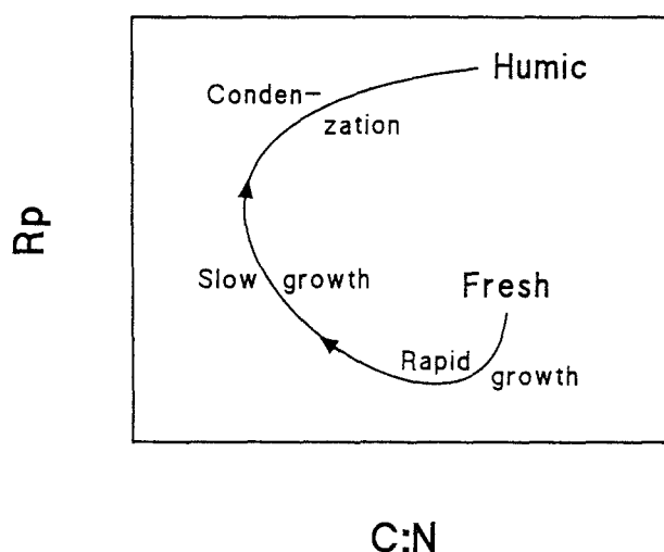
Fig. 12. Generalized R_p -C:N pattern of plant detritus during the decay sequence from fresh material to the end of humification. The 3 major decay phases are indicated; phase 1: Rapid growth, phase 2: Slow growth, phase 3: Condensation. Scales on the R_p and C:N axis and the shape of the curve may depend on the actual source material examined.
